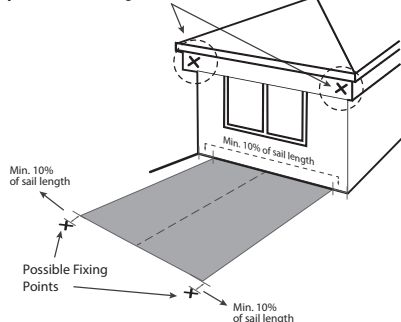
Fig. 1 Possible Fixing Points
