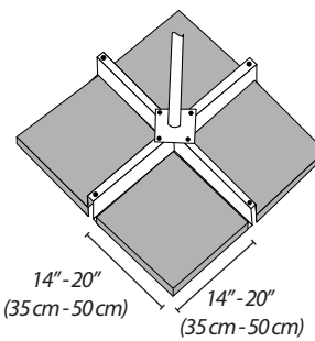
Option 1 - Position (4) - 14"-20" (35 cm - 50 cm) paver stones onto the base before raising canopy.
