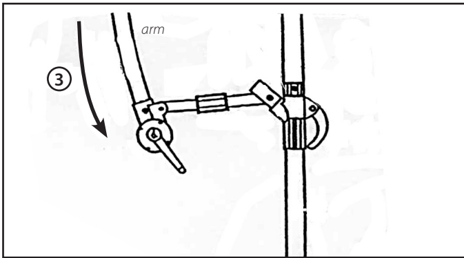
B. 3: Keeping the clamp lever locked (down) slowly lower arm to down position.
